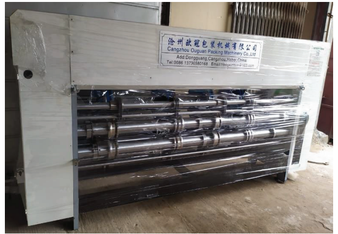
Figure 8: Combination Slotting Machine
